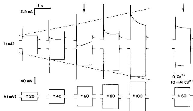
FIGURE 3 Records of voltage-dependent inward current present in a Type B photoreceptor are shown under conditions of 100 mM external Ba^{++} and K^+ current blockers ( 10 mM 4-AP, 100 mM TEA). From a holding potential of -60 mV, successive command steps in multiples of 20 mV reveal activation of an inward current at potentials more positive than -40 mV. This current increases nonlinearly, reaching its peak value at 0 mV (left arrow) and diminishes thereafter. Note that at 0 mV (absolute) the inward current decreases substantially from its maximum amplitude. Such a decrease was eliminated when substitution of Ba^{++} for Ca^{++} in the ASW was preceded by thorough washing with 0 Ca^{++} -ASW. From a holding potential of -60 mV, successive commands to potentials less than -60 mV elicit a non-voltage-dependent leak current, indicated by the lower dashed lines. The upper dashed line is extrapolated from potentials less than or equal to -50 mV. Note that when 10 mM Cd^{++} is substituted for Ca^{++} in the external bathing medium the current elicited by the command to 0 mV (absolute) begins to approach the extrapolated leak level (indicated by the dashed line).
